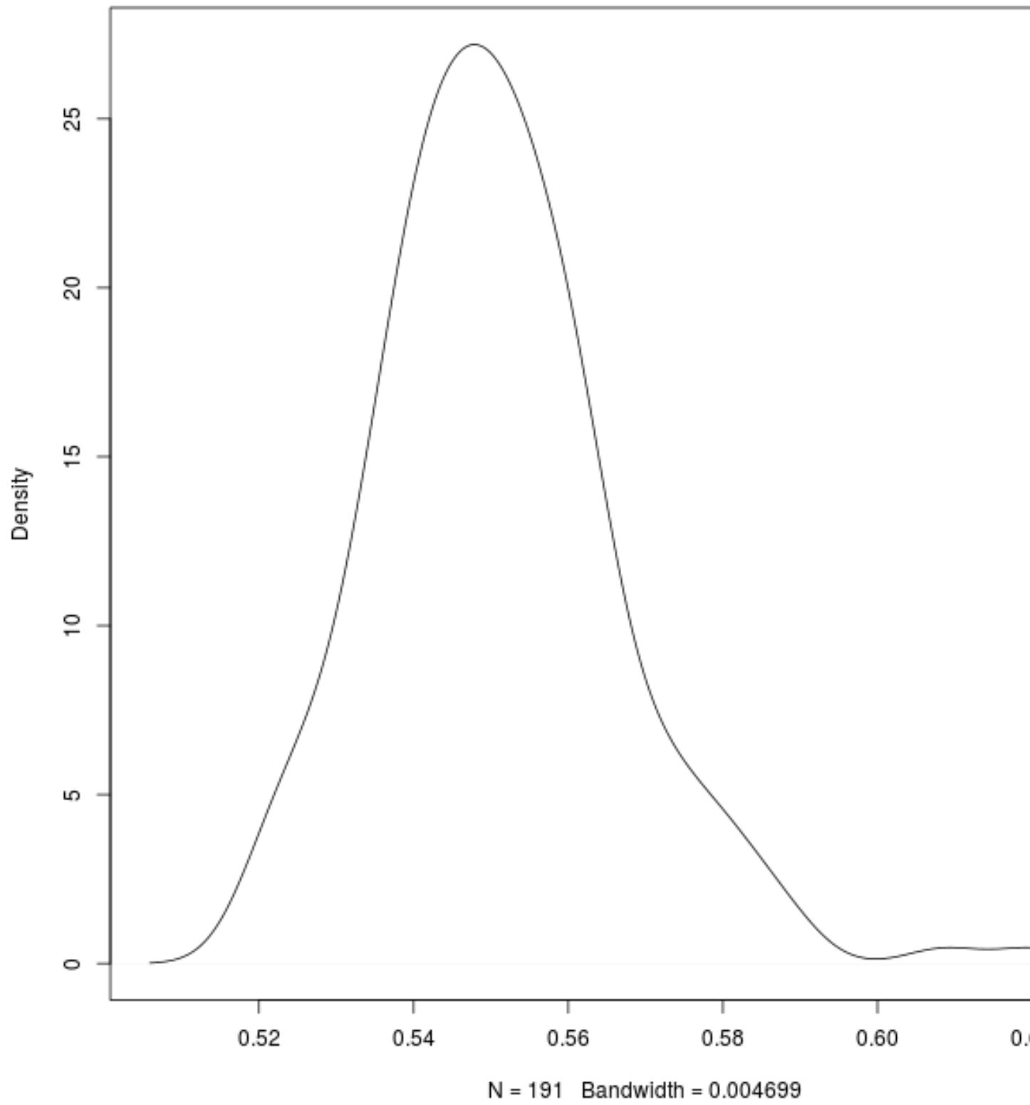
Figure 5: Example for a MDR plot
