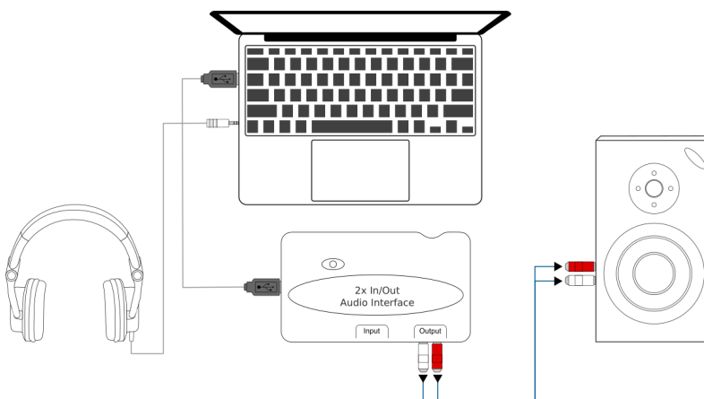
Figure2: Using Mixxx together with an external audio interface
